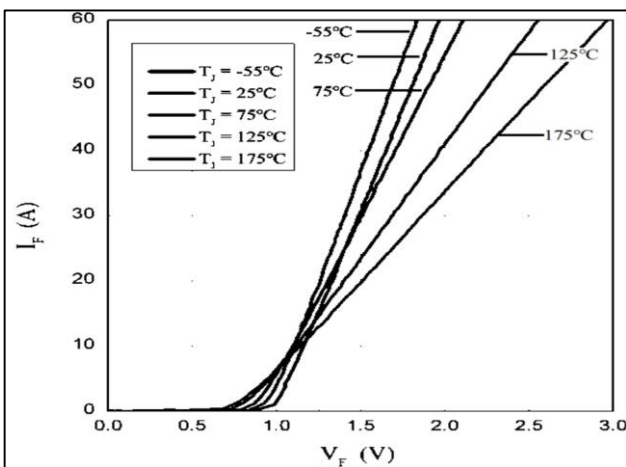
Diode Characteristic
